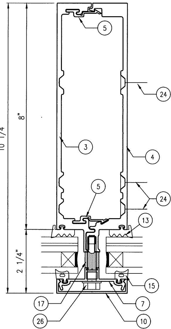
14 INTERMEDIATE VERTICAL 1-5/16" (Dry Glazed)
