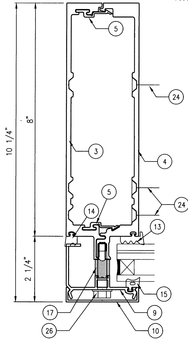
13 JAMB 1-5/16" (Dry Glazed)
