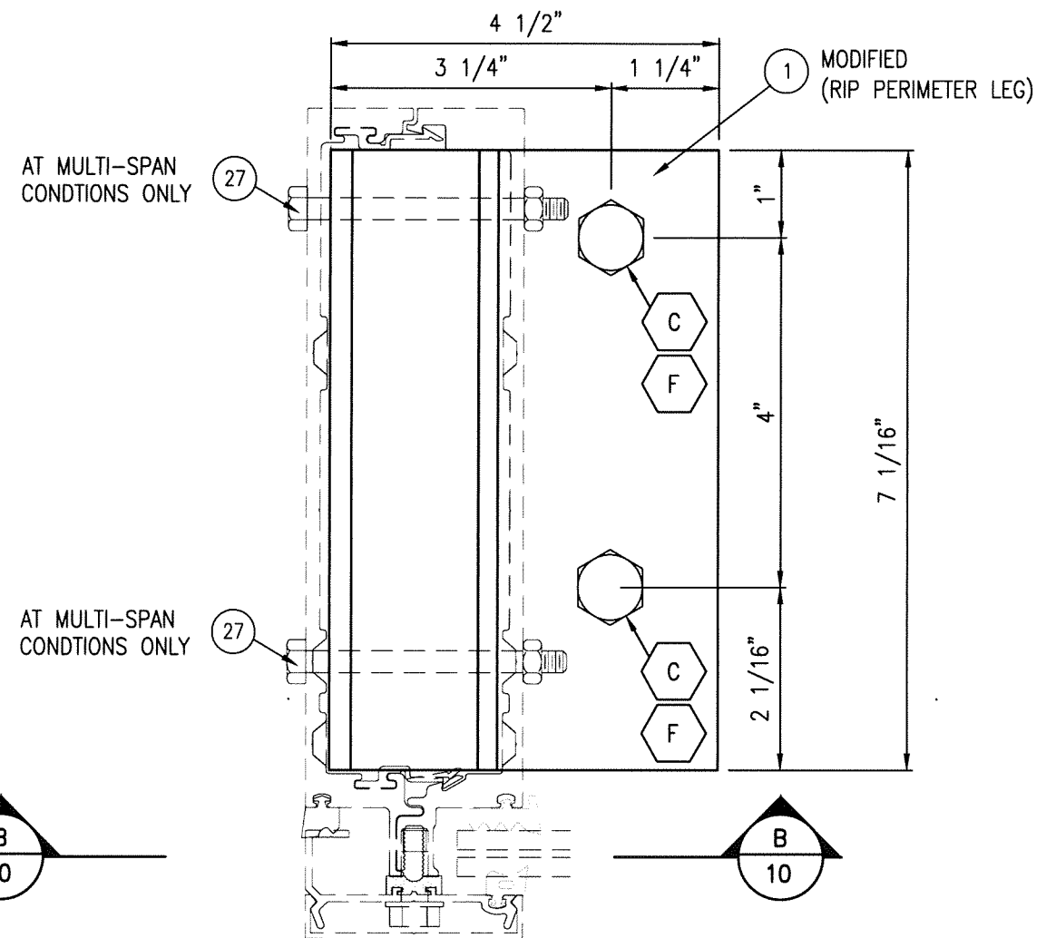
23 HEAD ANCHOR CLIP EXTRUDED ALUMINUM CLIP
