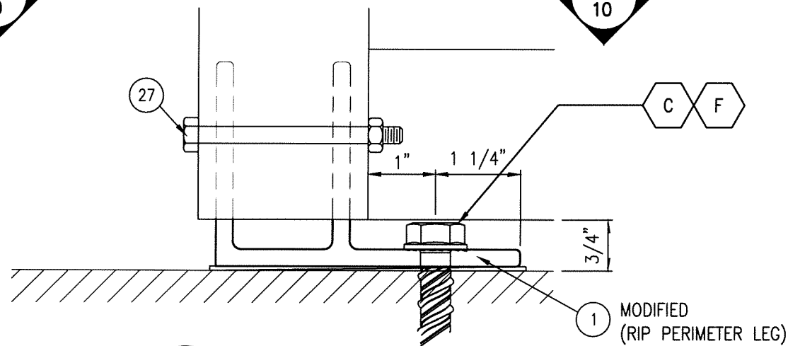
BB HEAD/SILL JAMB ANCHOR CLIP EXTRUDED ALUMINUM CLIP
