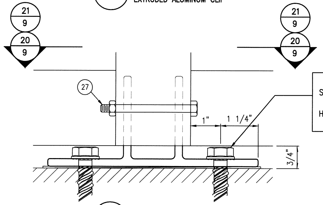
AA HEAD/SILL ANCHOR CLIP EXTRUDED ALUMINUM CLIP
