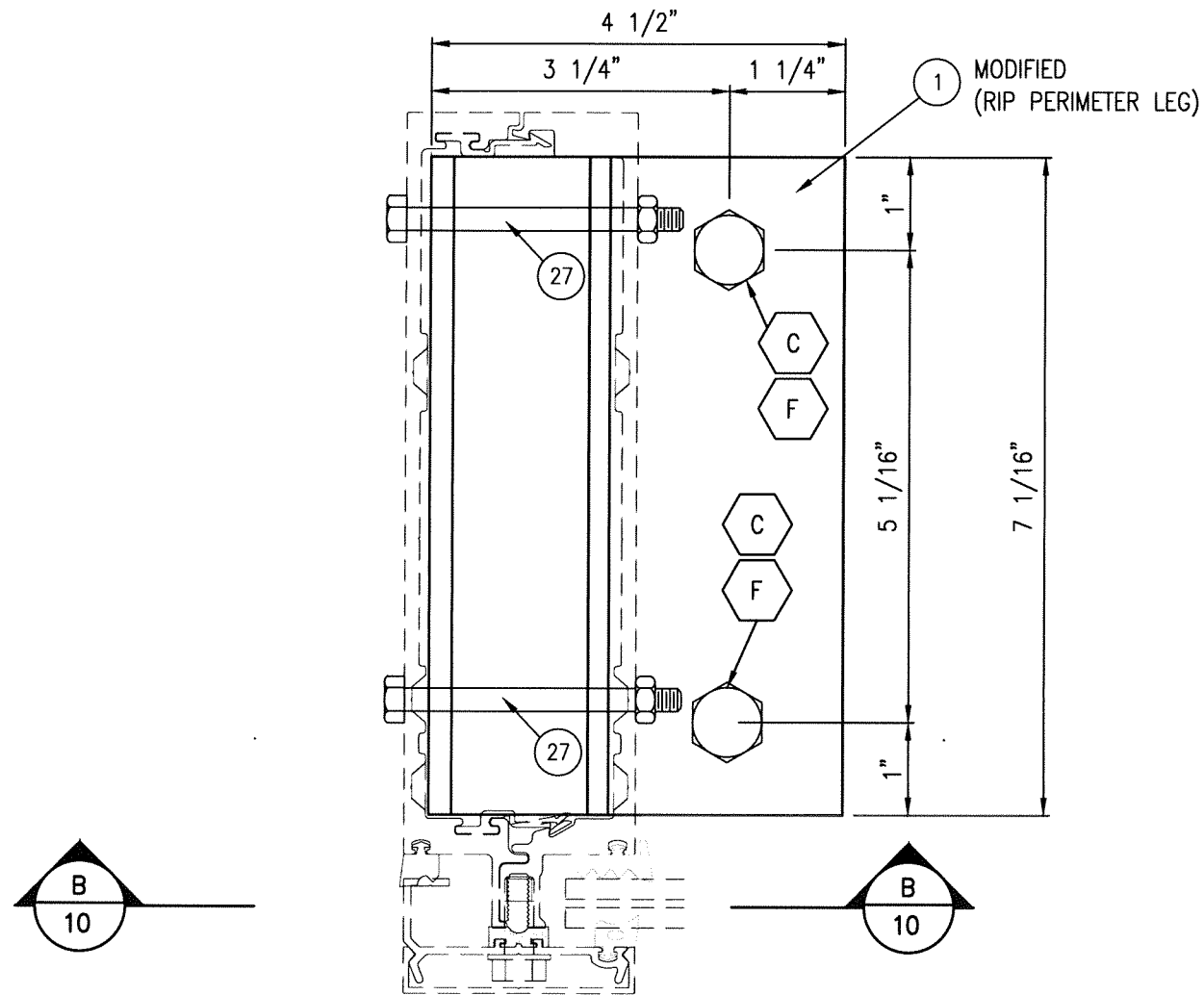
22 SILL ANCHOR CLIP EXTRUDED ALUMINUM CLIP
